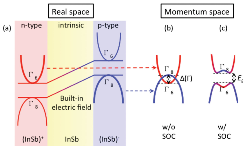
Figure 3. a) Schematic band structure and real space potential alignment of p-i-n junction between the InSb layers with positively charged bonds and negatively charged bonds as (InSb) + and (InSb) - , respectively. b) The resulting k -space band structure with a band inversion at the \Gamma point (without SOC), and c) the excitation gap opened by SOC. The bands with red and blue colors denote their origin from (InSb) + and (InSb) - , respectively.
