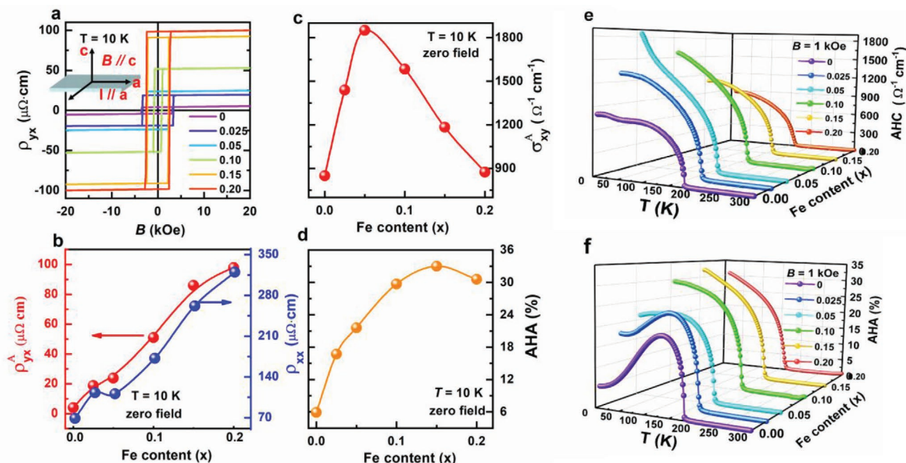
Figure 2. AHE subsequent to Fe doping. a) Hall resistivity \rho_{yx} as a function of magnetic field B at 10 K for B // c and I // a . b) Fe-doping dependences of anomalous Hall resistivity \rho_{yx}^A and longitudinal resistivity \rho_{xx} . c) and d) Fe-doping dependences of AHC \sigma_{xy}^A and AHA, respectively, at 10 K and zero field. e, f) Temperature dependence of AHC and AHA values of \text{Co}_{3-x}\text{Fe}_x\text{Sn}_2\text{S}_2 at a field of 1 kOe.
