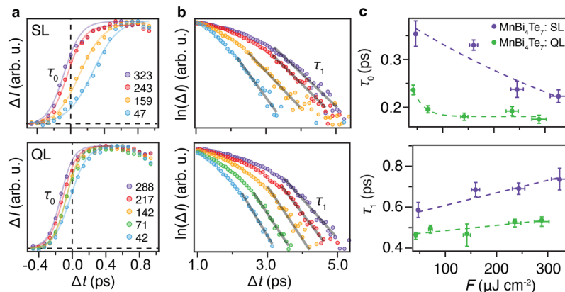
Figure 4. Charge transfer and phonon relaxation in MnBi 4 Te 7 . (a, b) (E, k) -integrated intensity difference from 0 to 70 meV above E_F and from -0.2 to 0.2 \text{\AA}^{-1} for SL and QL terminations of MnBi 4 Te 7 . Each data set was acquired with the fluence stated in (a) in units of \mu\text{J}/\text{cm}^2 . In (a) we examine the rising edge of the signal (circles), representing the filling of unoccupied states above E_F , and fit a sigmoid function (curves) to extract the time scale \tau_0 of the filling. In (b) we analyze the decay part of the signal on a logarithmic intensity scale and perform exponential fits (lines) to extract the phonon relaxation time scale \tau_1 . (c) Extracted time scales from (a) and (b) as a function of laser fluence. Dashed curves provide a guide to the eye.
